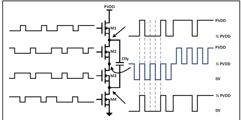
Figure 4: Multi-level amplifier output stage
