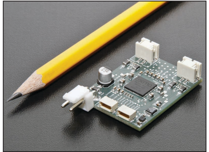
Photo 1: Ultra-compact amplifier design made possible
