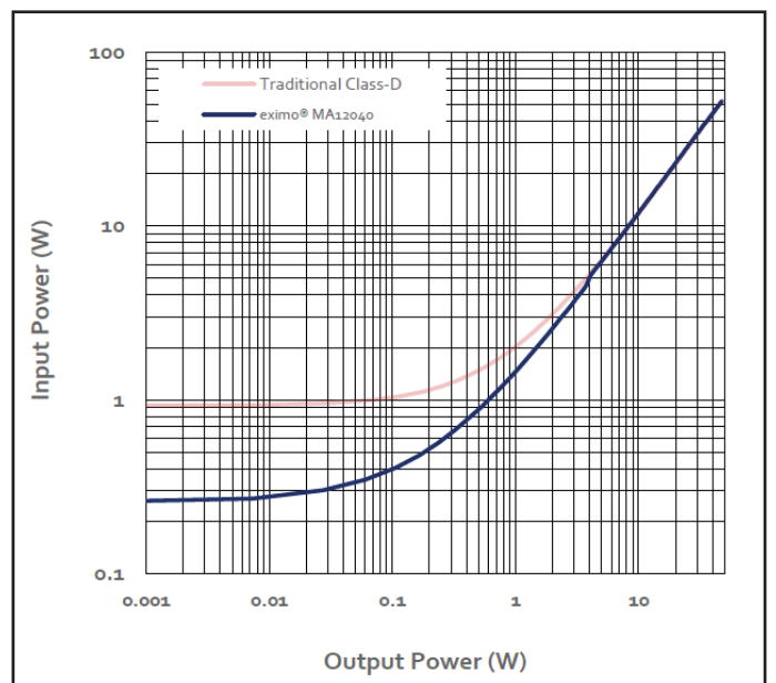
Figure 8: Input power vs. output power
