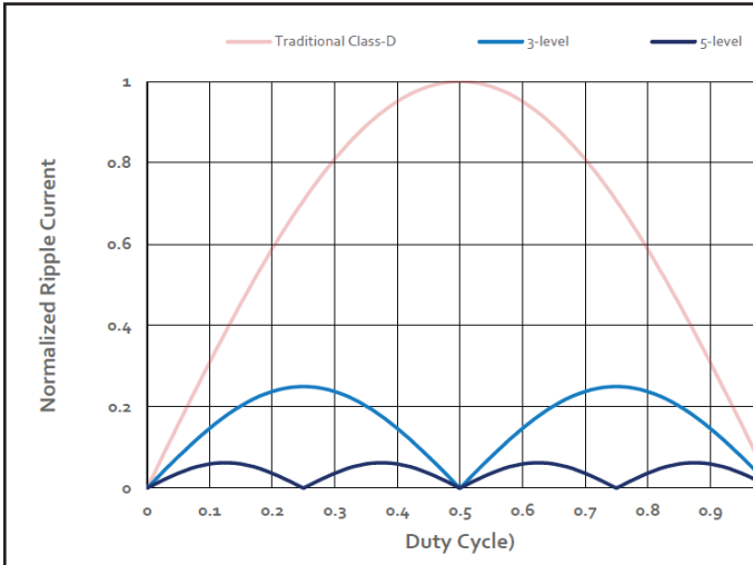
Figure 6: Normalized ripple currents vs. duty cycle
