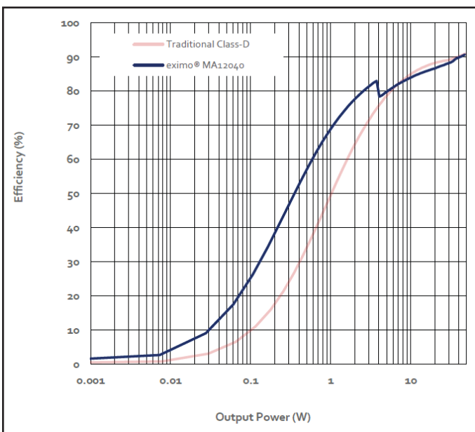
Figure 7: Efficiency vs. output power
