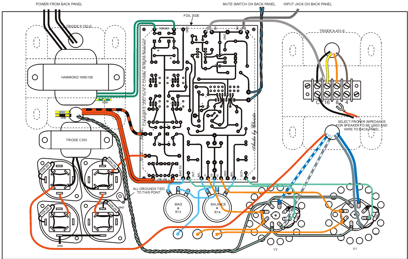
Figure 5 - Chassis Wiring for Hybrid Amplifier
